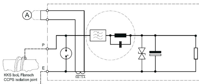
Basic circuit diagram
